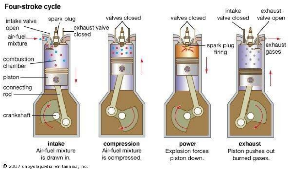
Fig. Cycle of operation in four stroke engine
