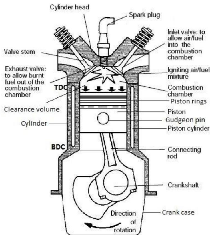
Fig.( Different parts of IC engine)
